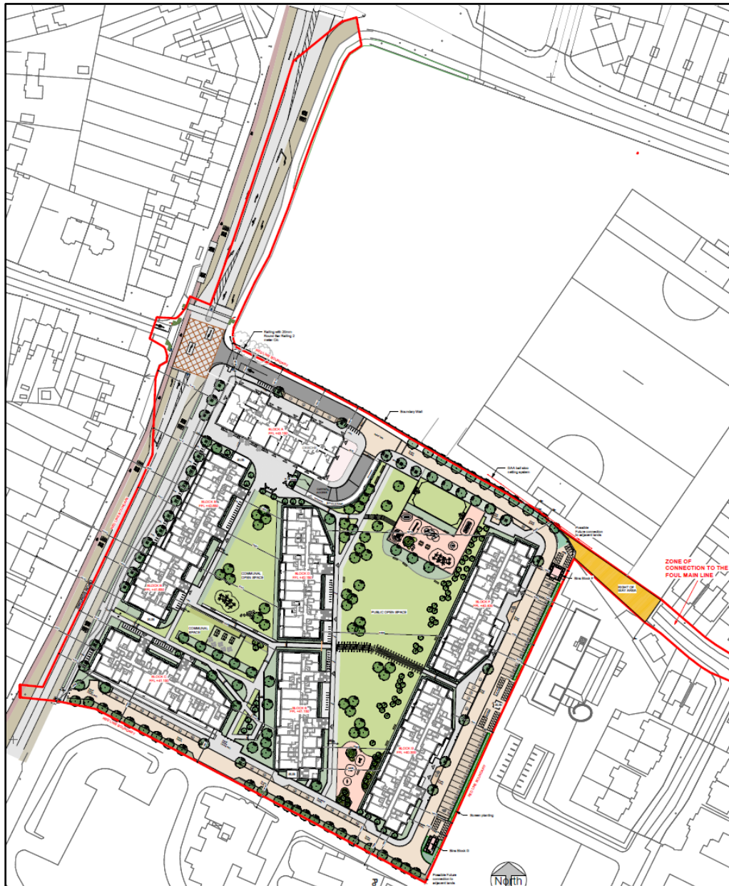
Figure 4.1 Proposed Site Layout
